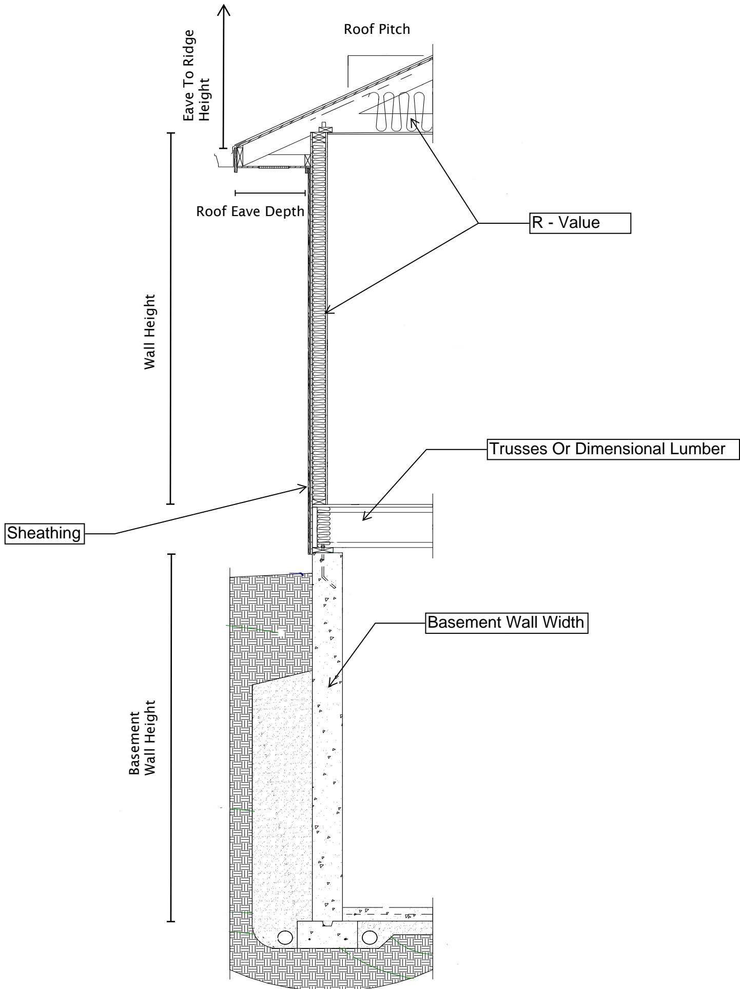
FIRST FLOOR & BASEMENT WALL SECTION DETAIL
