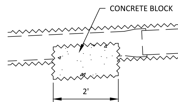
AERIAL SANITARY SEWER STABILIZER BLOCK NOT TO SCALE
