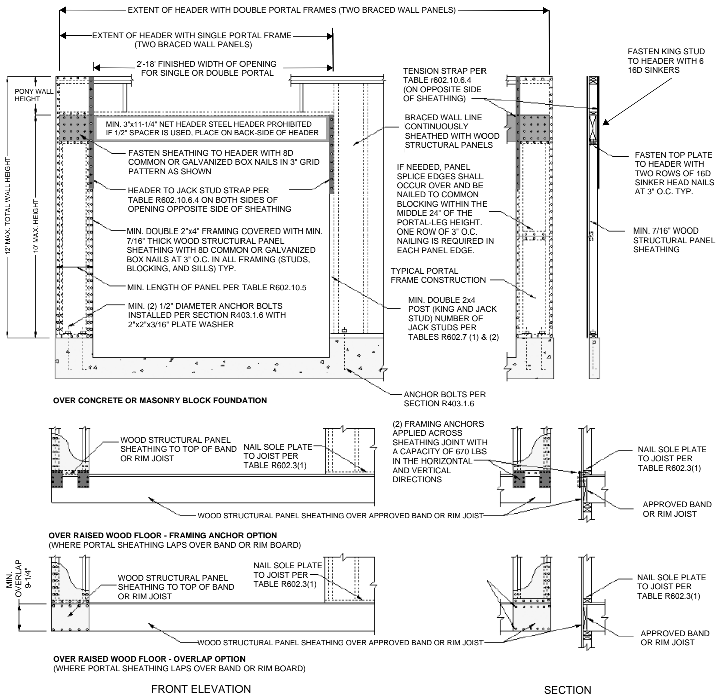
Figure R602.10.6.4 – CONTINUOUSLY SHEATHED PORTAL FRAME
